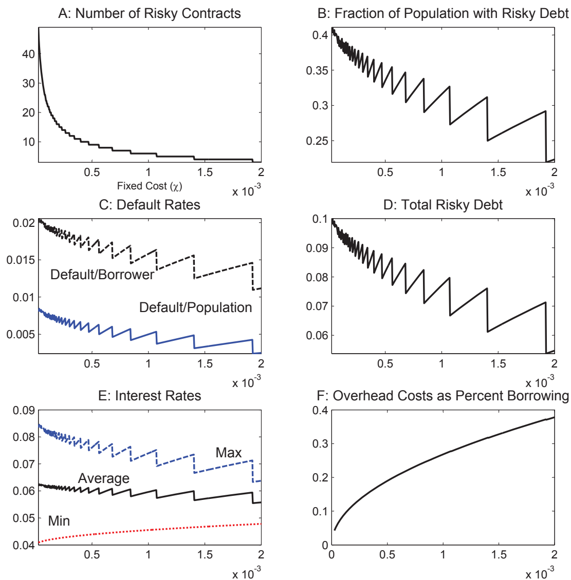
Figure 4: Varying the Fixed Cost
