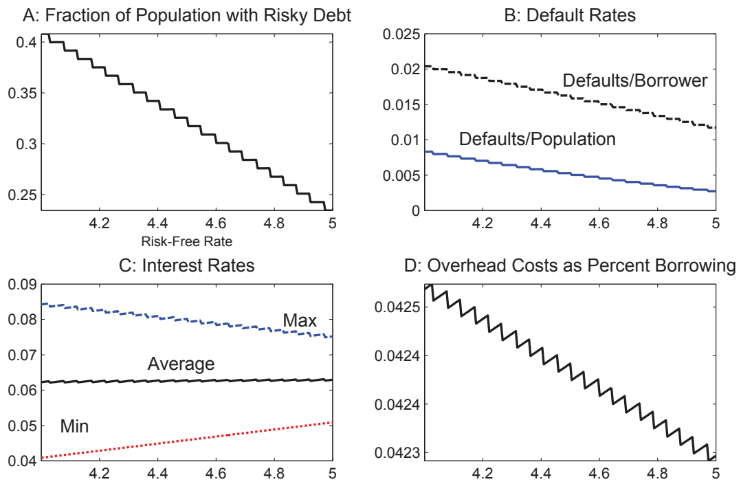
Figure 5: Varying the Interest Rate
