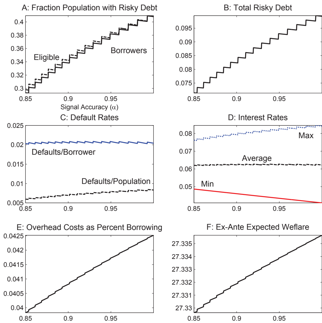
Figure 6: Varying the signal accuracy
