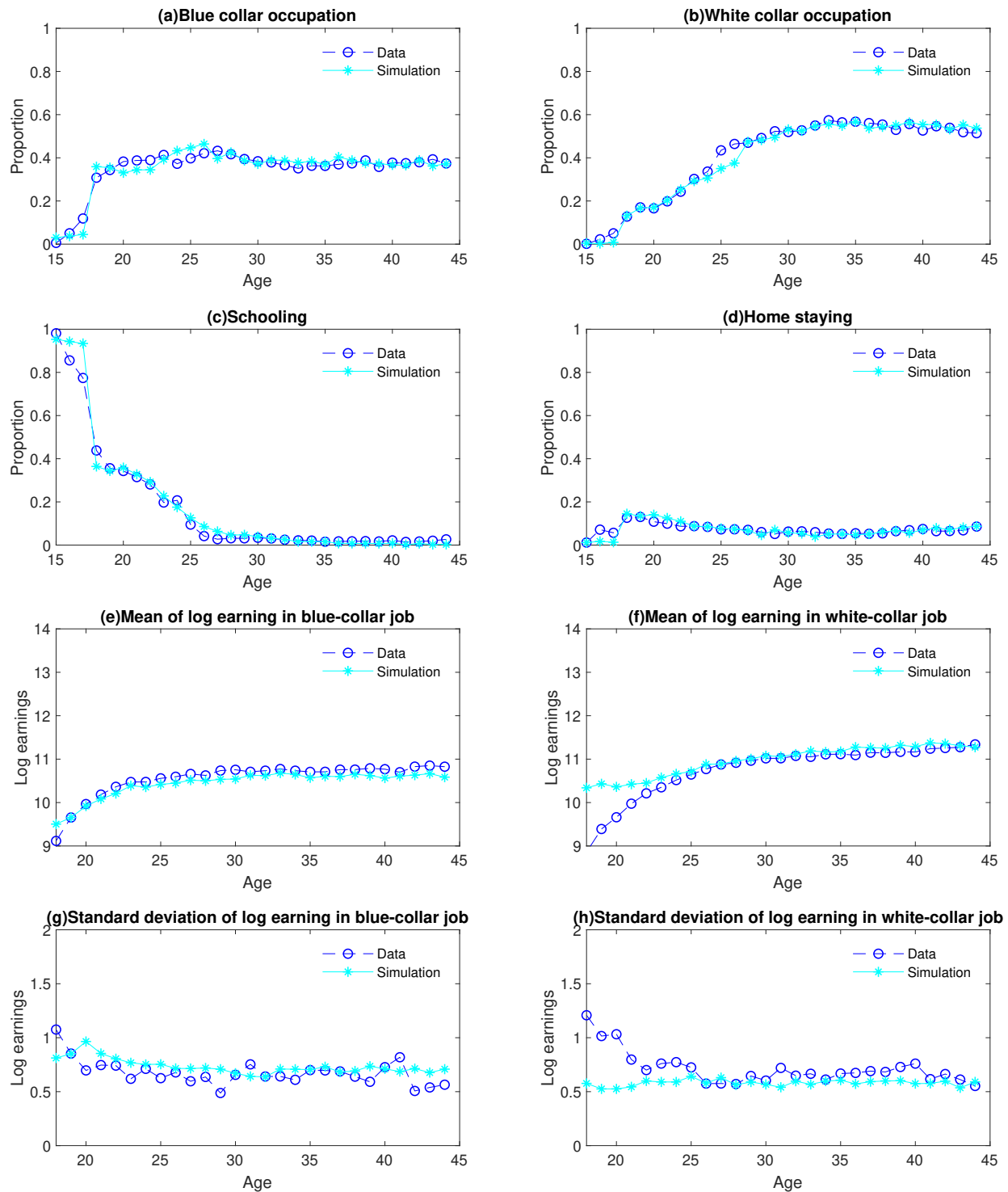
Figure 5: The comparison of choice distribution and earning profile between real data and model simulations
