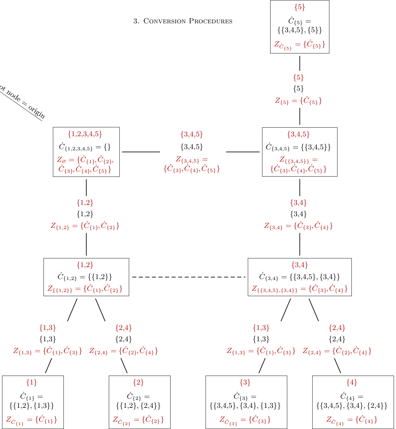
FIGURE 2. An outcome-set form (top row), converted into a choice-set form (middle row), and converted again into an outcome-set form (bottom row). The two outcome-set forms are equivalent by renaming outcomes.
